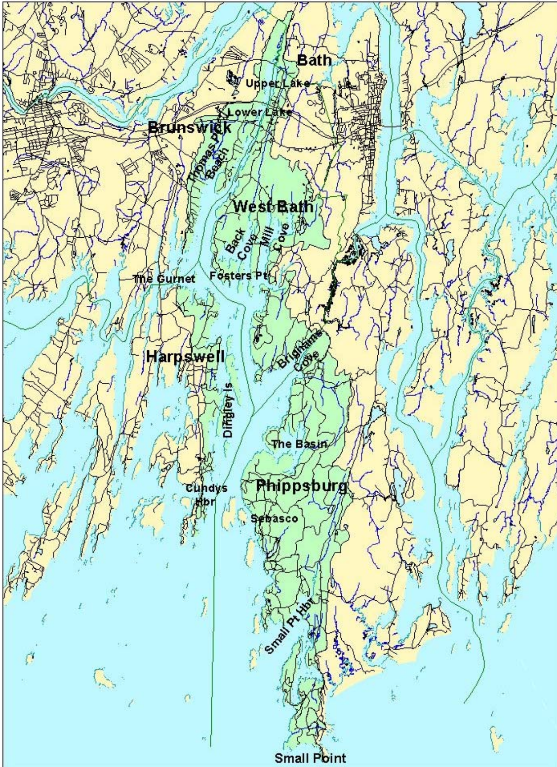
Figure 1. New Meadows River watershed
