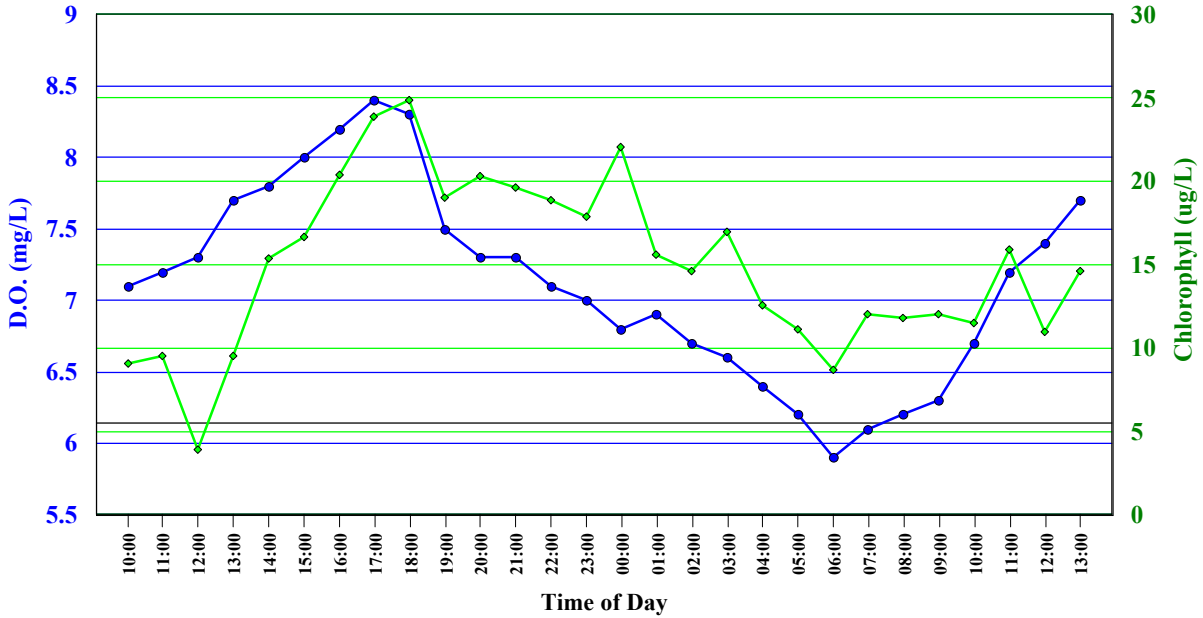
Figure 13. Diurnal relationship between dissolved oxygen concentration and chlorophyll at station NM6
