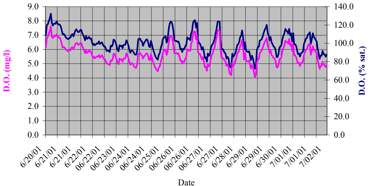
Figure 14. Diurnal fluctuations in D.O concentration and saturation at station NMM over a 12-day period
